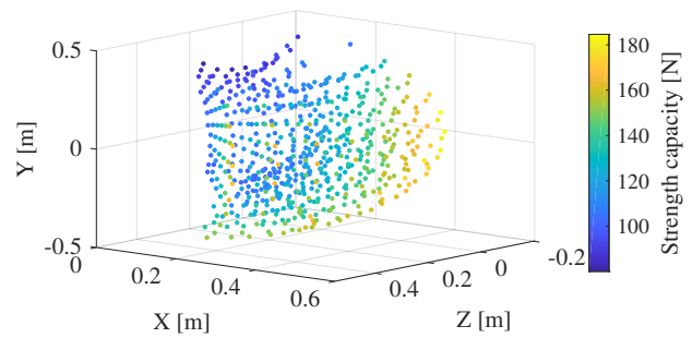
Fig. 4. Strength capacity (N) with respect to the distance (m) from the centre of the thorax.
