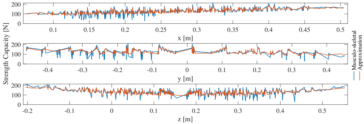
Fig. 3. Strength capacity [N] estimated with the musculo-skeletal model (in blue) and with the approximated model (in orange) with respect to the distance [m] from the centre of the thorax.
