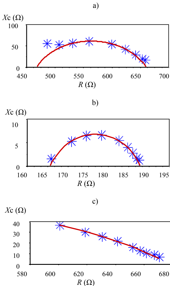
Figure 3. Fitting of raw data taken with a Seca mBCA 525.
