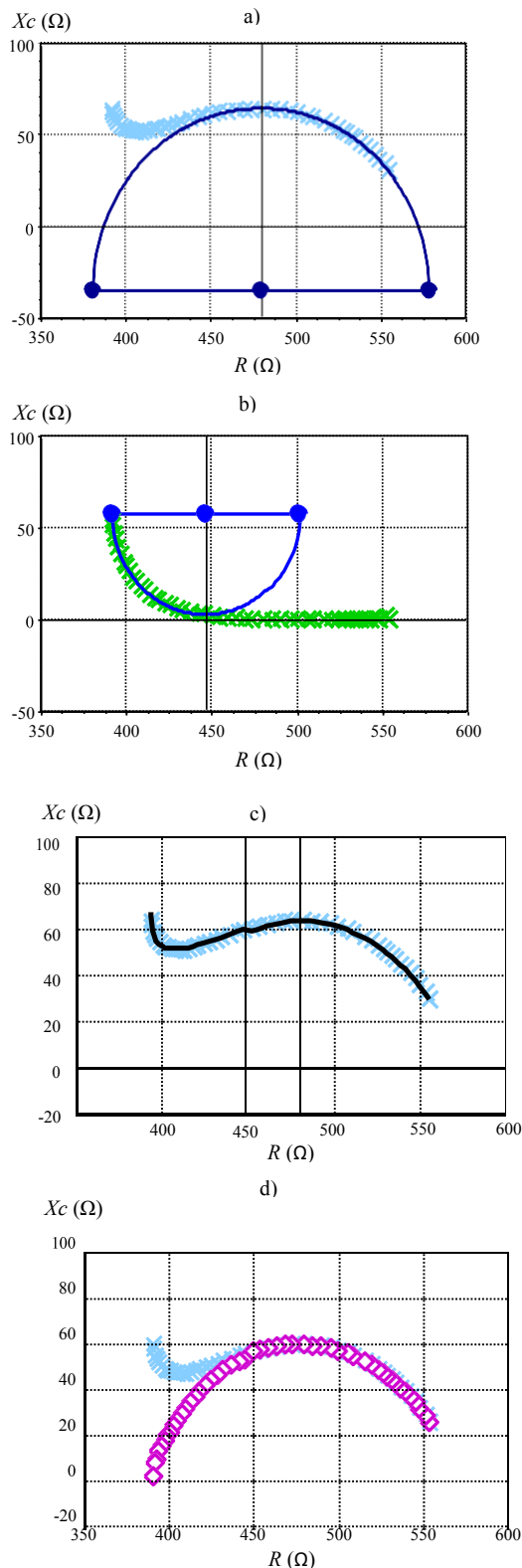
Figure 1. Fitting of raw data using two dispersions. a) Main dispersion obtained with the values at 10, 20 and 50 kHz; b) fitting for the values obtained by subtracting the corresponding theoretical values from the raw data at frequencies where the hook effect is visible (in this case, beginning with 90 kHz, where the difference between raw and theoretical data is 2.5 \Omega ); c) overall fitting of the raw data by adding the values corresponding to the two dispersions considered in this article.
