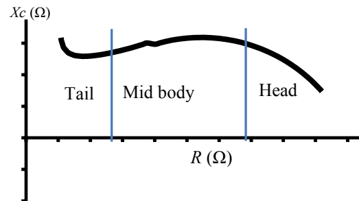
Figure 2. “S” shape form of ebis data showing the so called “hook” effect.
